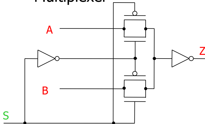
Multiplexer
