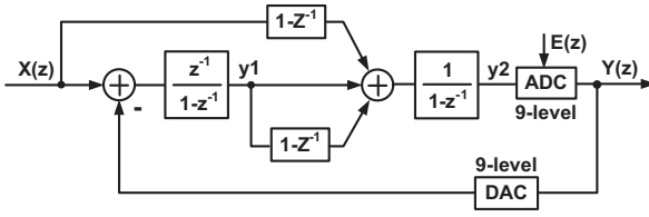
Fig. 3. Proposed second-order feedforward \Delta\Sigma AD modulator.
