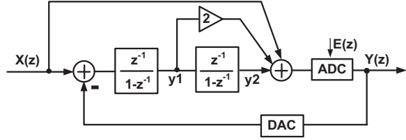
Fig. 2. Conventional second-order feedforward \Delta\Sigma AD modulator.
