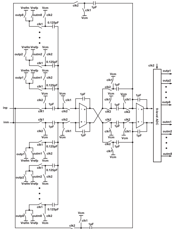
Fig. 6. Switched-Capacitor implementation of proposed feedforward \Delta\Sigma AD modulator.
