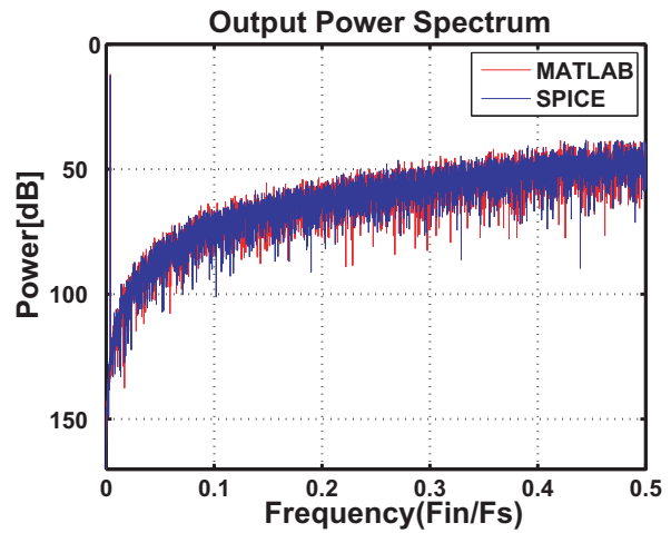
Fig. 8. Compared output power spectrum of proposed multibit \Delta\Sigma AD modulator.
