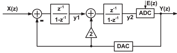
Fig. 1. Second-order feedback \Delta\Sigma AD modulator.
