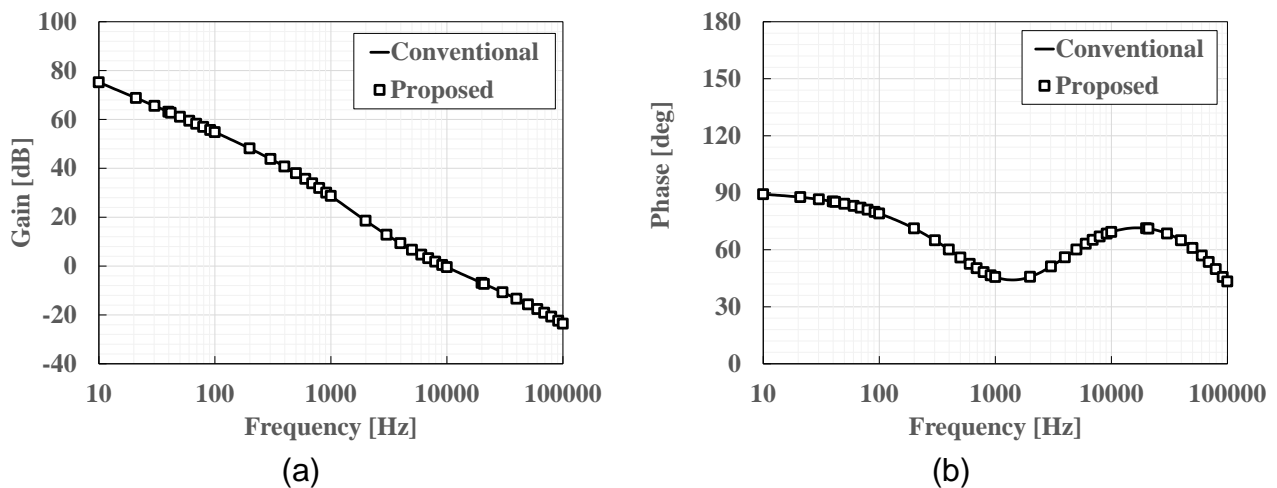
Fig. 5. Comparison of loop gain in Fig. 3. (a) Gain. (b) Phase.
