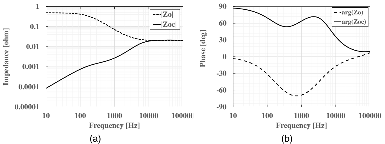
Fig. 4. Simulation result of Z_o and Z_{oc} in Fig. 3 (b). (a) Impedance. (b) Phase.
