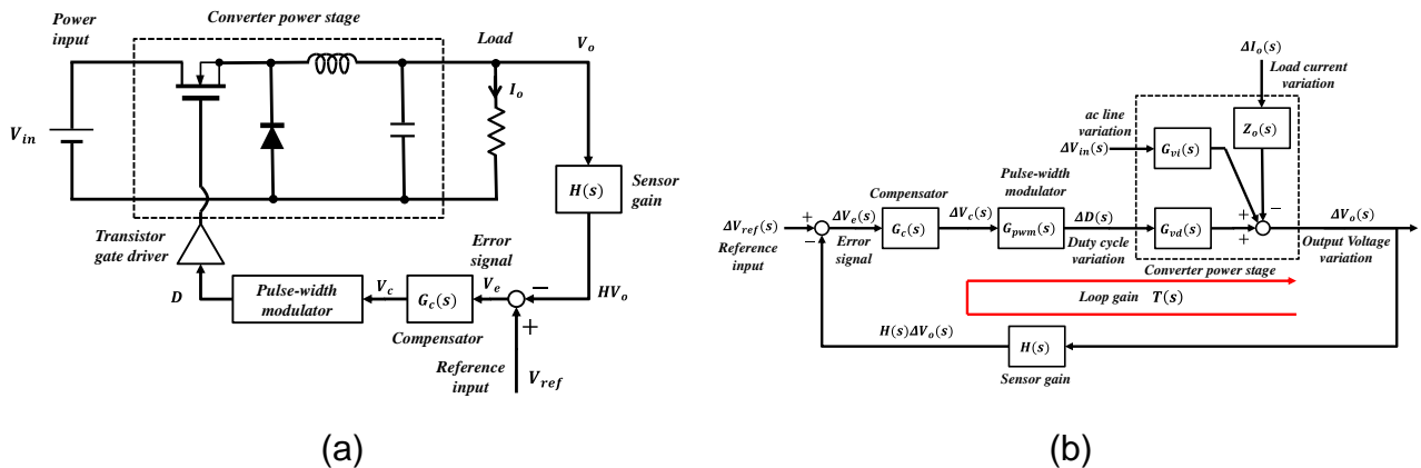
Fig. 2. Feedback loop for regulation of the output voltage in dc-dc buck converter. (a) Feedback loop block diagram. (b) Functional block diagram of the feedback system [2].
