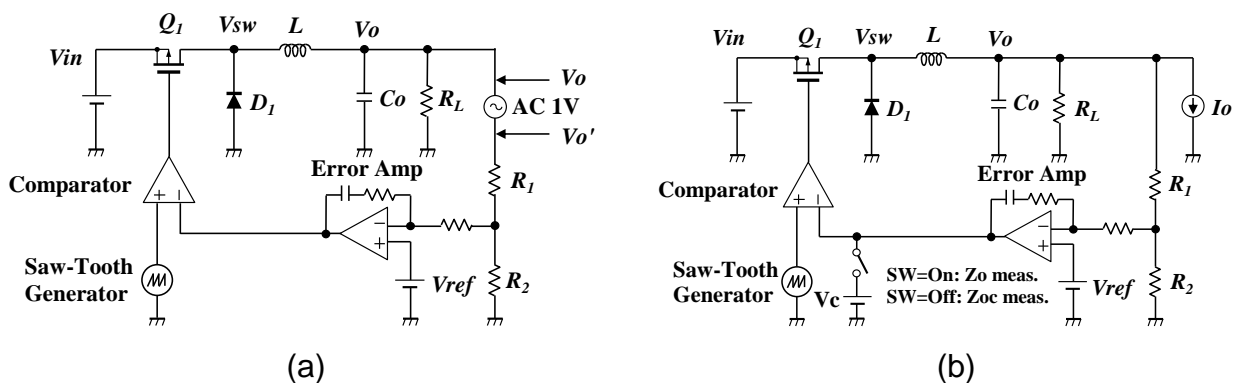
Fig. 3. Simulation circuit for measuring the loop gain. (a) Conventional loop gain measurement circuit. (b) Z_o and Z_{oc} measurement circuit.
