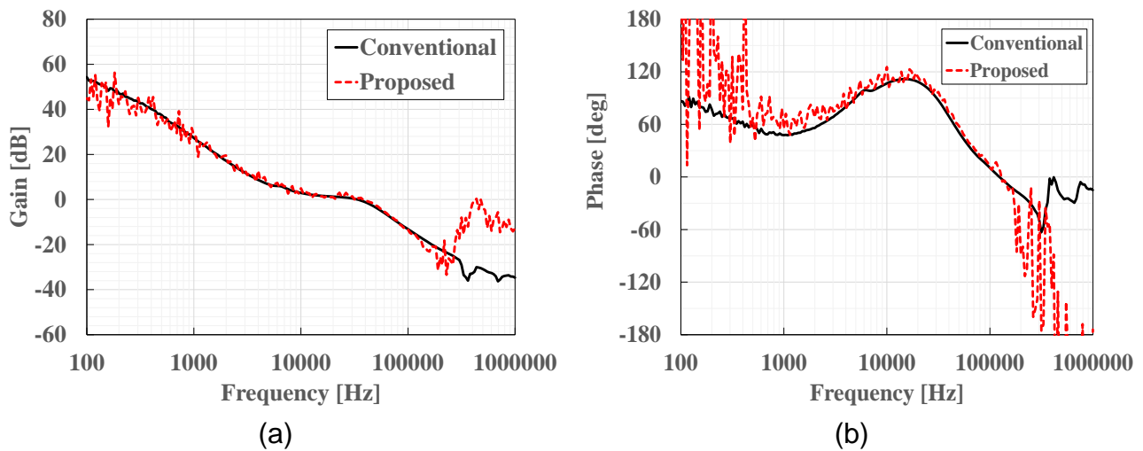
Fig. 6. Comparison of loop gain in experiment. (a) Gain. (b) Phase.
