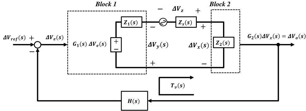
Fig. 1. Measurement of loop gain by voltage injection [1,2].
