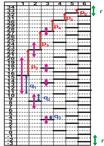
Fig. 3. Redundant search algorithm of a 5-bit SAR ADC with 6 steps (case 1).
