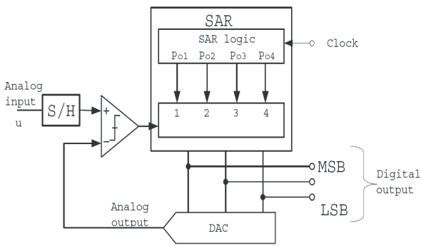
Fig. 1. Block diagram of an SAR ADC.
